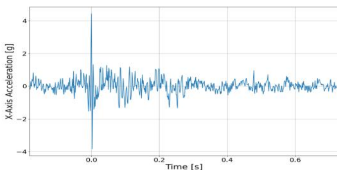
Figure 1. Impact event time-domain data
