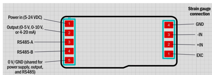
Figure 5: Solder terminal connections to device
