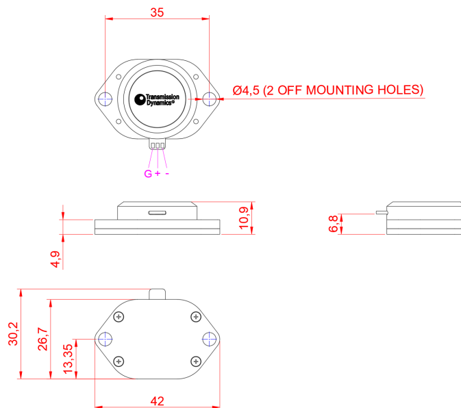
Figure 3: MiniTemp Dimensions
